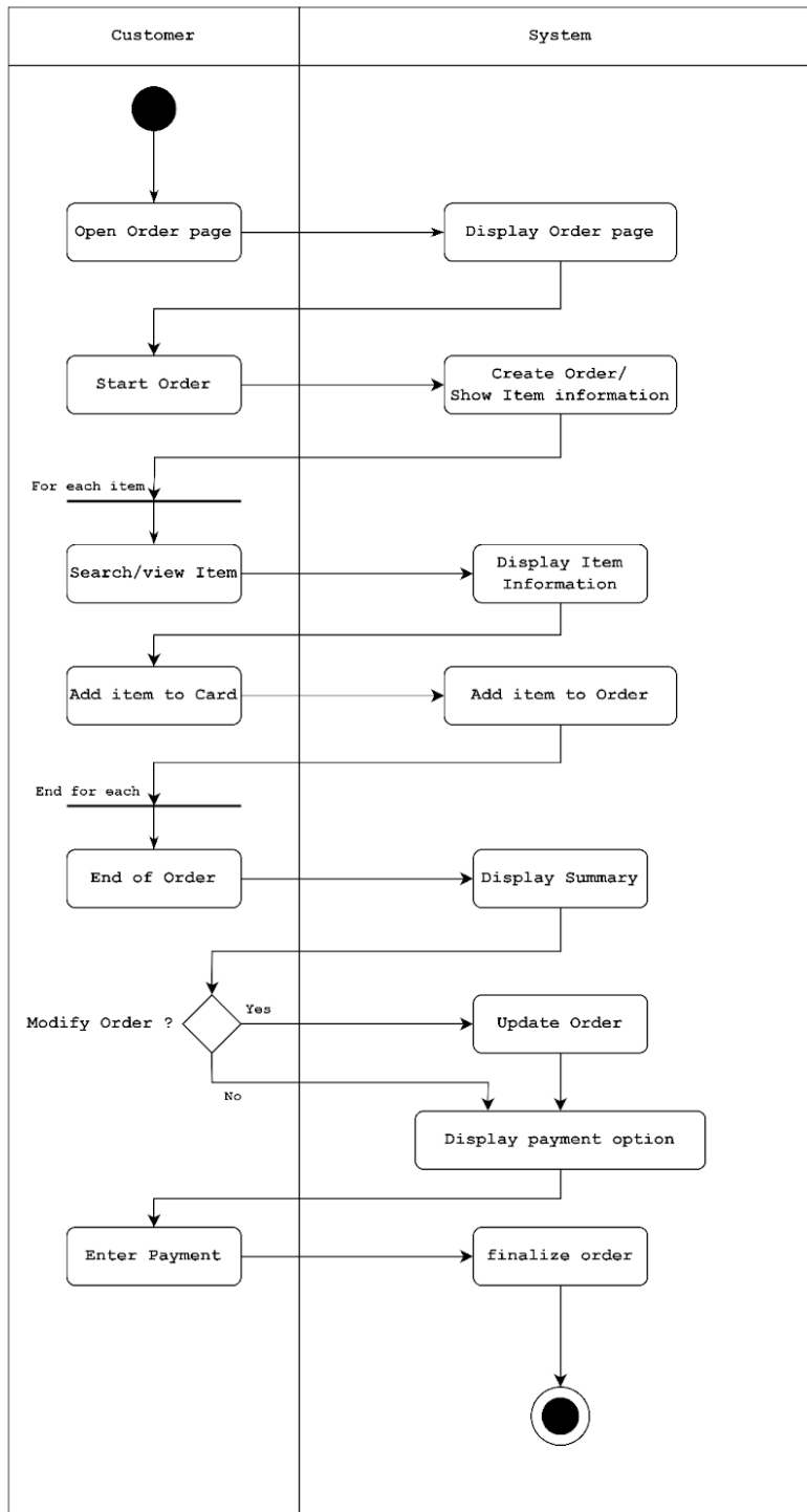
Activity Diagram : Customer Create Online order.
