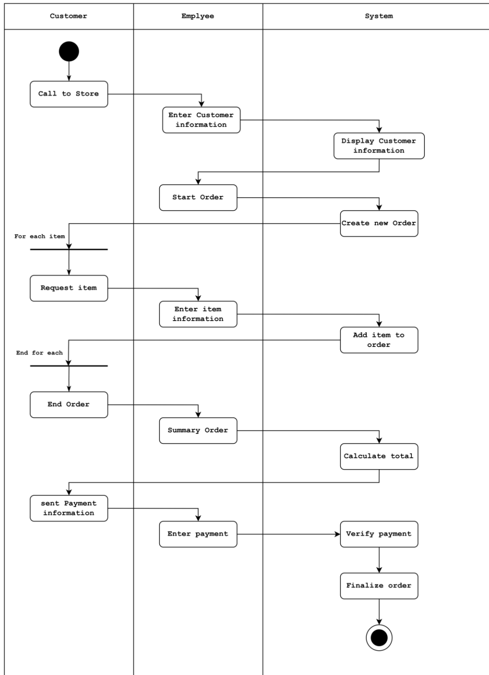
Activity Diagram : Employee create telephone order.
